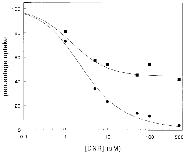
Fig. 6. Inhibition by high daunorubicin concentrations of the ATP-dependent GS-DNP and GSSG uptake into membrane vesicles from GLC4/ADR cells. The uptake of 10 nM [ ^3 H]GS-DNP (■) and [ ^3 H]GSSG (●) was measured at different concentrations of daunorubicin. Uptake without DNR was set at 100%.
