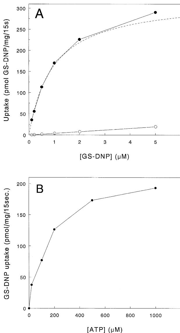
Fig. 2. ATP and GS-DNP concentration dependence of the ATP-dependent GS-DNP uptake into membrane vesicles of GLC4/ADR cells. Uptake of [ ^3 H]GS-DNP into membrane vesicles of GLC4/ADR in 15 s was measured at different GS-DNP concentrations, ranging from 20 to 5000 nM GS-DNP, with (●) or without (○) 1 mM of ATP (A) and at different ATP concentrations, ranging from 20 to 1000 \mu M ATP, at 5 \mu M GS-DNP (B). The dashed line (upper panel) indicates the ATP-dependent uptake of GSDNP, obtained by subtracting the uptake of GS-DNP in the absence of ATP (lower curve) from the uptake in the presence of ATP (upper curve). Data are from a representative experiment.
