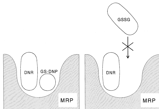
Fig. 7. Model of the binding pocket of MRP explaining non-competitive inhibition of GS-DNP transport and competitive inhibition of GSSG transport by DNR.
