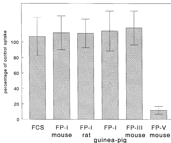
Fig. 3. Interaction of polyclonal antisera with the ATP-dependent GS-DNP uptake into membrane vesicles from GLC4/ADR cells. The ATP-dependent uptake in 15 s of 10 nM [ ^3 H]GS-DNP into membrane vesicles from GLC4/ADR cells was measured with no additions (100%), fetal calf serum (FCS) and serum from mice, a rat and a guinea pig which had been immunized with the fusion proteins FP-I, FP-III and FP-V [20,21].
